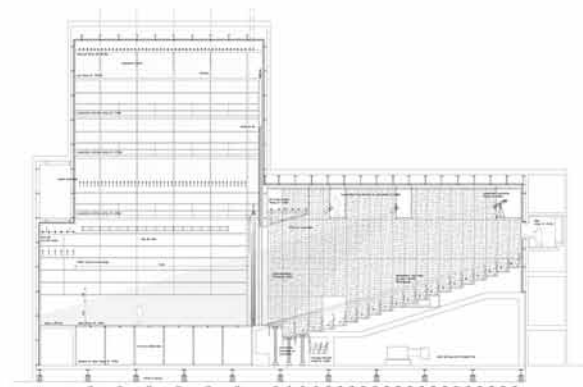
SECTION B-B (1/1000) - 12345
